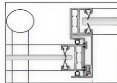
CLOSING SIDE
