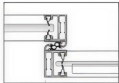
OPENING SIDE
